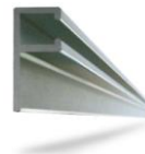
F-TR - 'F' section aluminium track 2,600mm long, 784 g/length
