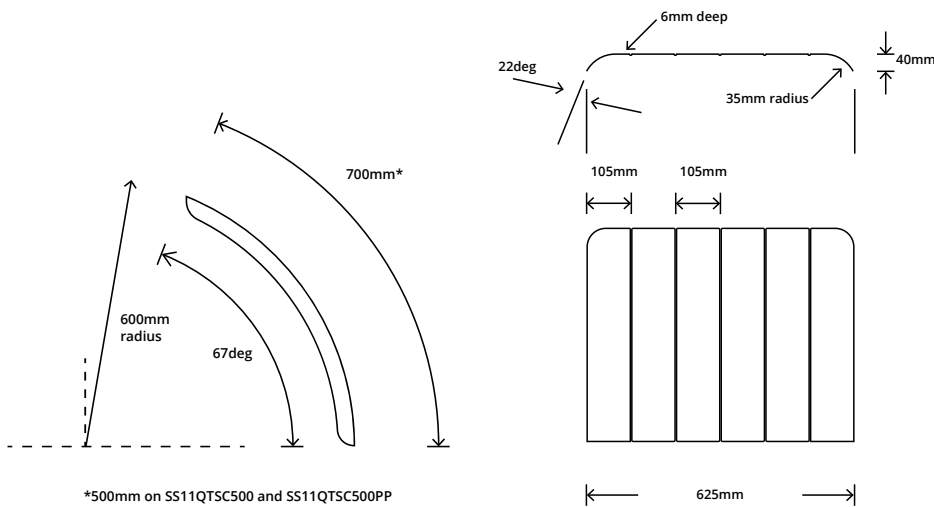
*500mm on SS11QTSC500 and SS11QTSC500PP
