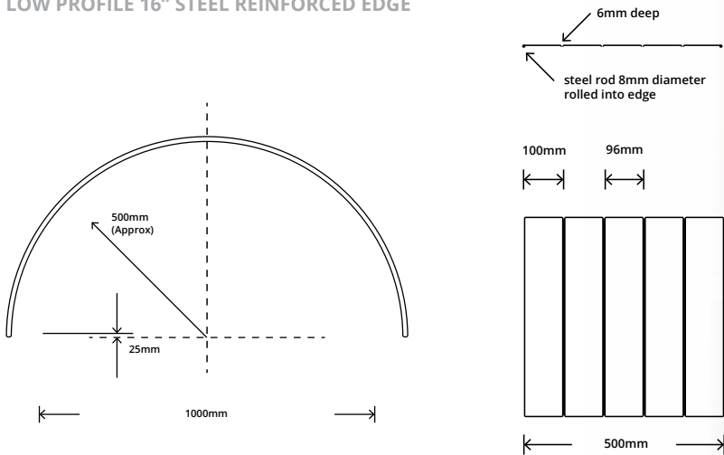
LOW PROFILE 16" STEEL REINFORCED EDGE
