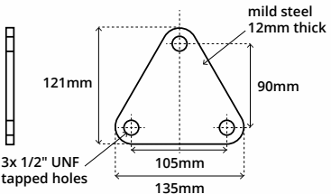
Optional part SP1 Sub Plate
